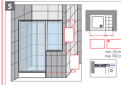
Profilo chiuso / Closed profiles
