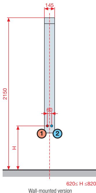
Wall-mounted version
