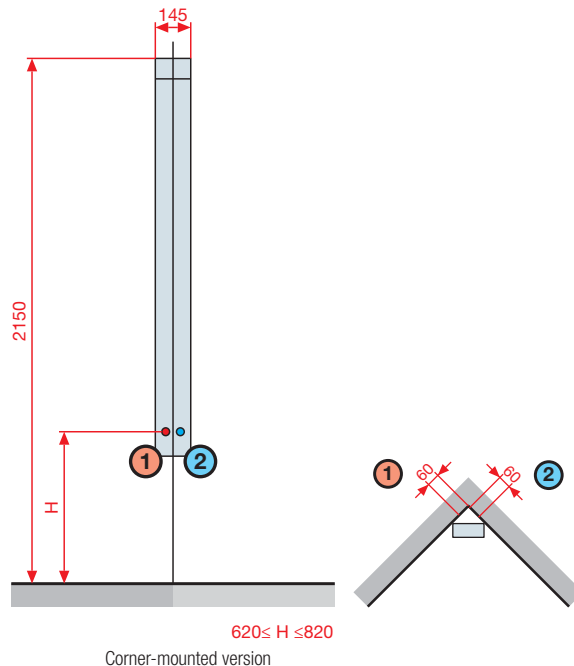
Corner-mounted version
