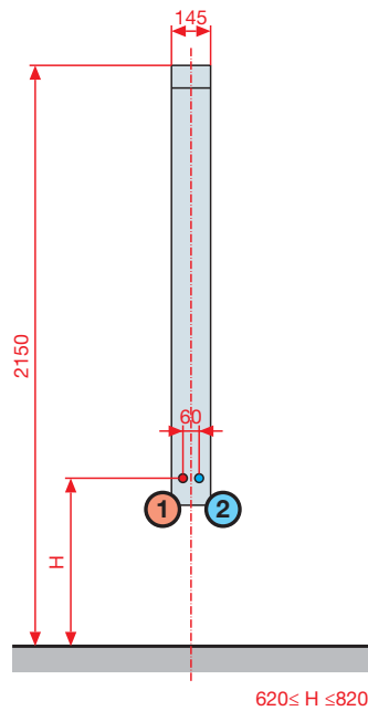
Standard Version
