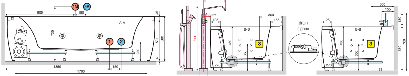
Floor-mounted mixer
