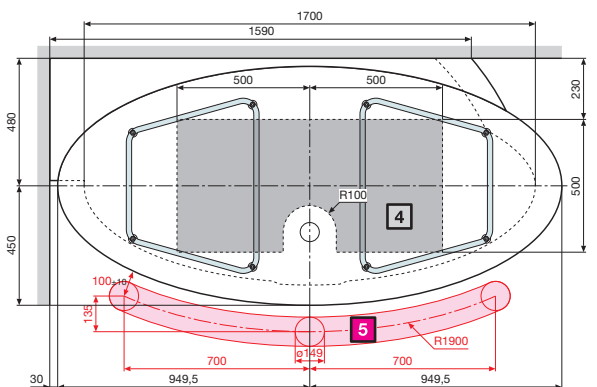
Floor-mounted mixer
