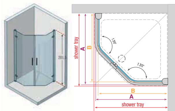
ref. 7 Murano Pentagono - Pentagon enclosure, 2 hinged doors
