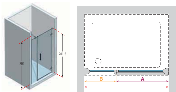
ref. 5 Murano G+F in line - In line hinged door and fixed panel for recess
