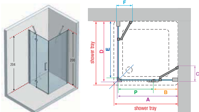
ref. 8 Coral G+F - Hinged door and side panel
