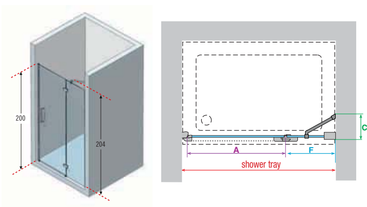
ref. 7 Coral 1B - Hinged door for recess
