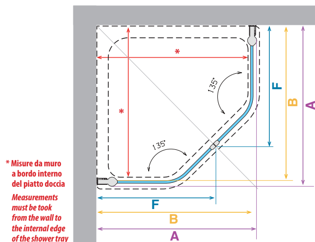
ref. 7 Giada Pentagono Cabina doccia pentagonale a 2 battenti Pentagon enclosure, 2 hinged sections
