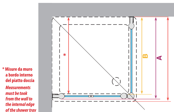
ref. 3 Giada F Fisso per Giada 2B e 1B Side panel for Giada 2B and 1B
