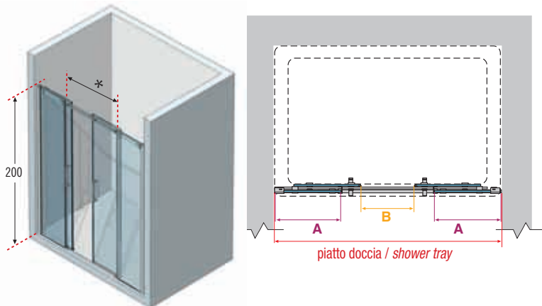
ref. 5 Diamanti 2A - Porta doccia a 2 ante, 1 scorrevole + 1 fissa in nicchia / 2 section door, 1 sliding + 1 fixed for recess
