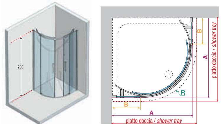
ref. 2 Diamanti R - Box doccia curvo a 4 ante, 2 scorrevoli + 2 fisse / Curved shower enclosure, 4 sections, 2 sliding + 2 fixed
